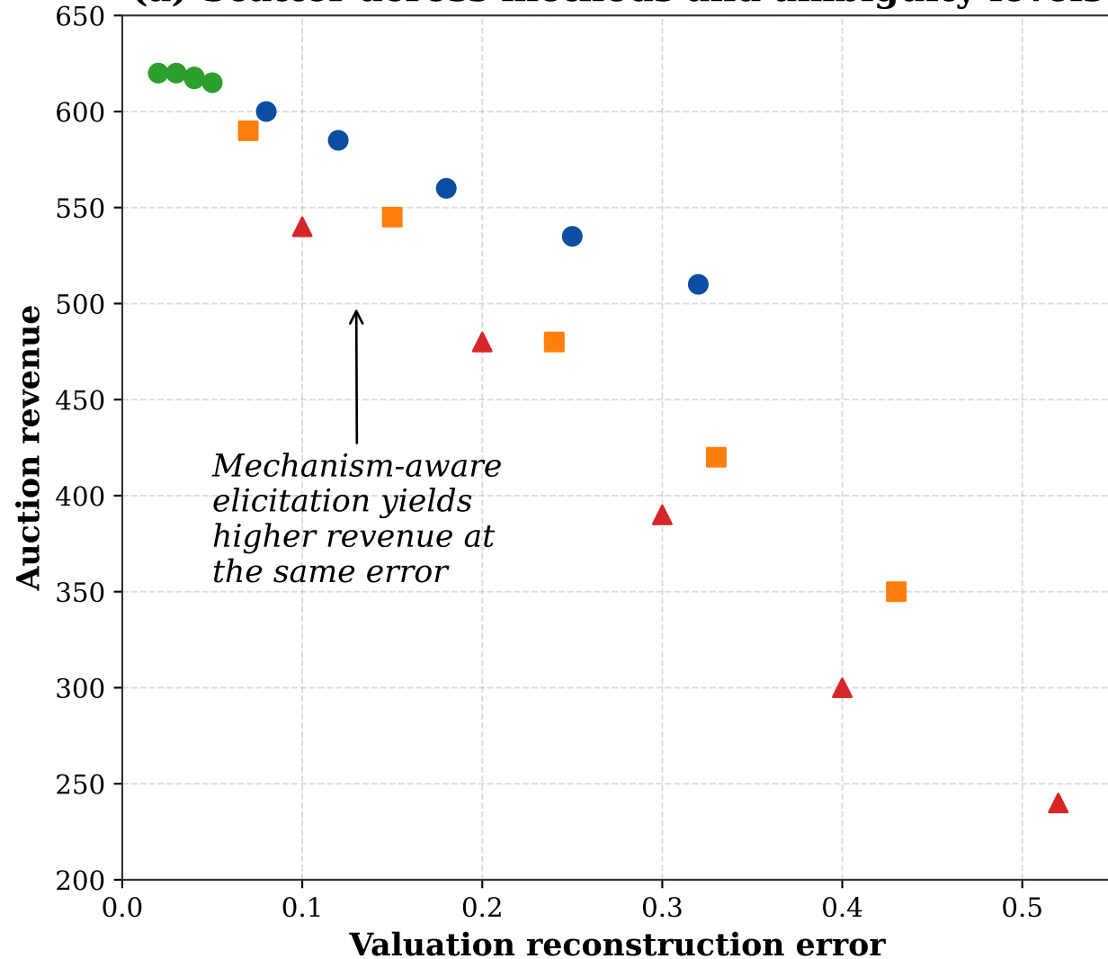
(a) Scatter across methods and ambiguity levels
